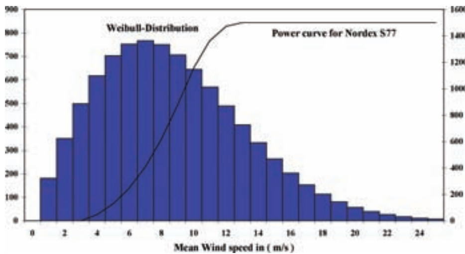
Figure 5. Wind speed frequency distribution throughout the year in the site depending on estimated data by WASP program and the power curve for the 1500 kW selected wind machine.
