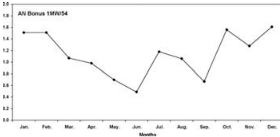
Figure 4. Monthly variation of the mean wind turbine efficiency for a commercial wind turbine 1000 kW during the year at Ras Benas Station.
