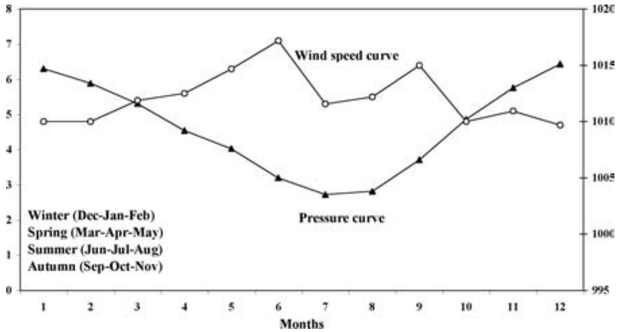
Figure 2. Monthly variation of the wind speed and air pressure depending on measured data at Ras Benas station.
